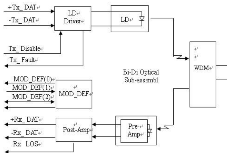
Block Diagram
