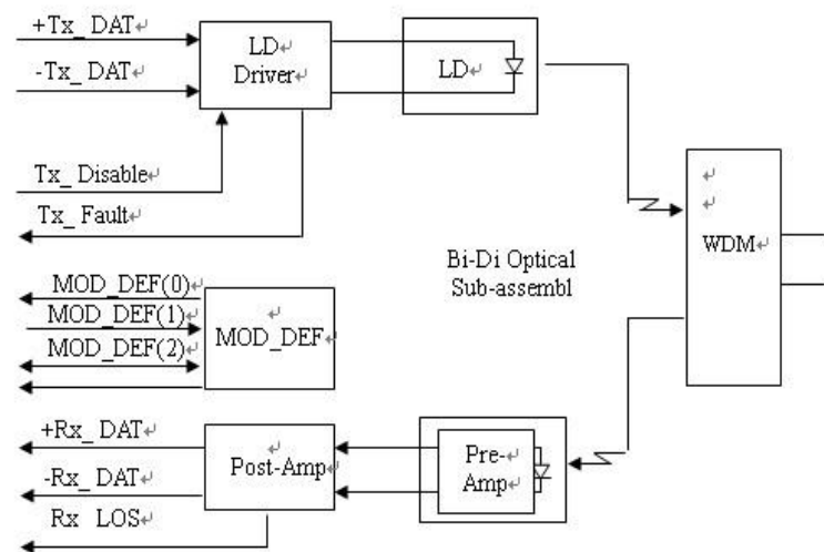
Block Diagram
