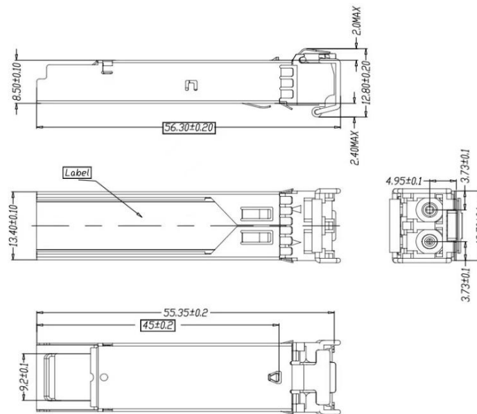
Mechanical Drawing
