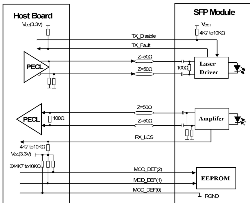
SFP Host Recommended Circuit
