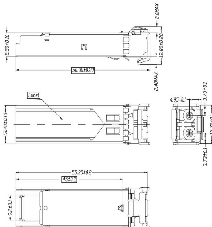
Mechanical Drawing
