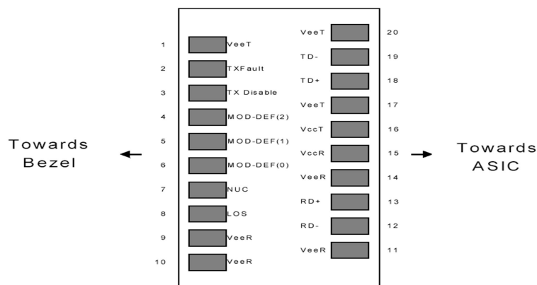
Diagram of Host Board Connector Block Pin Numbers and Names
