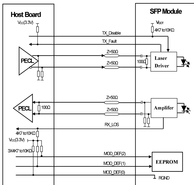
SFP Host Recommended Circuit
