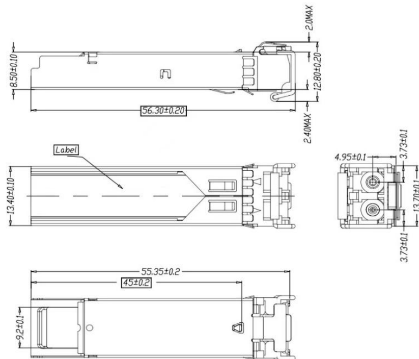
Mechanical Drawing
