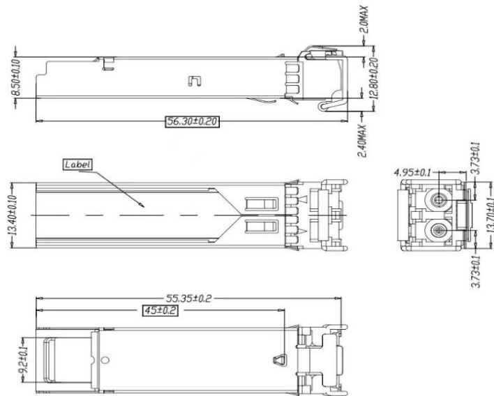
Mechanical Drawing
