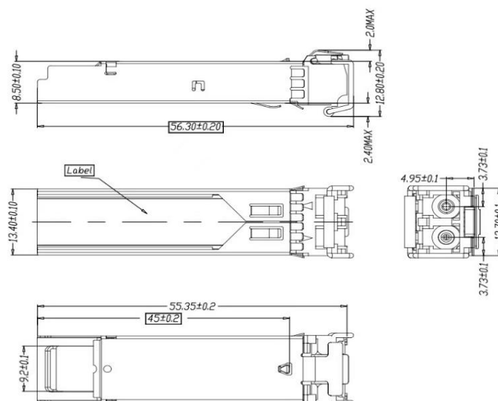
Mechanical Drawing
