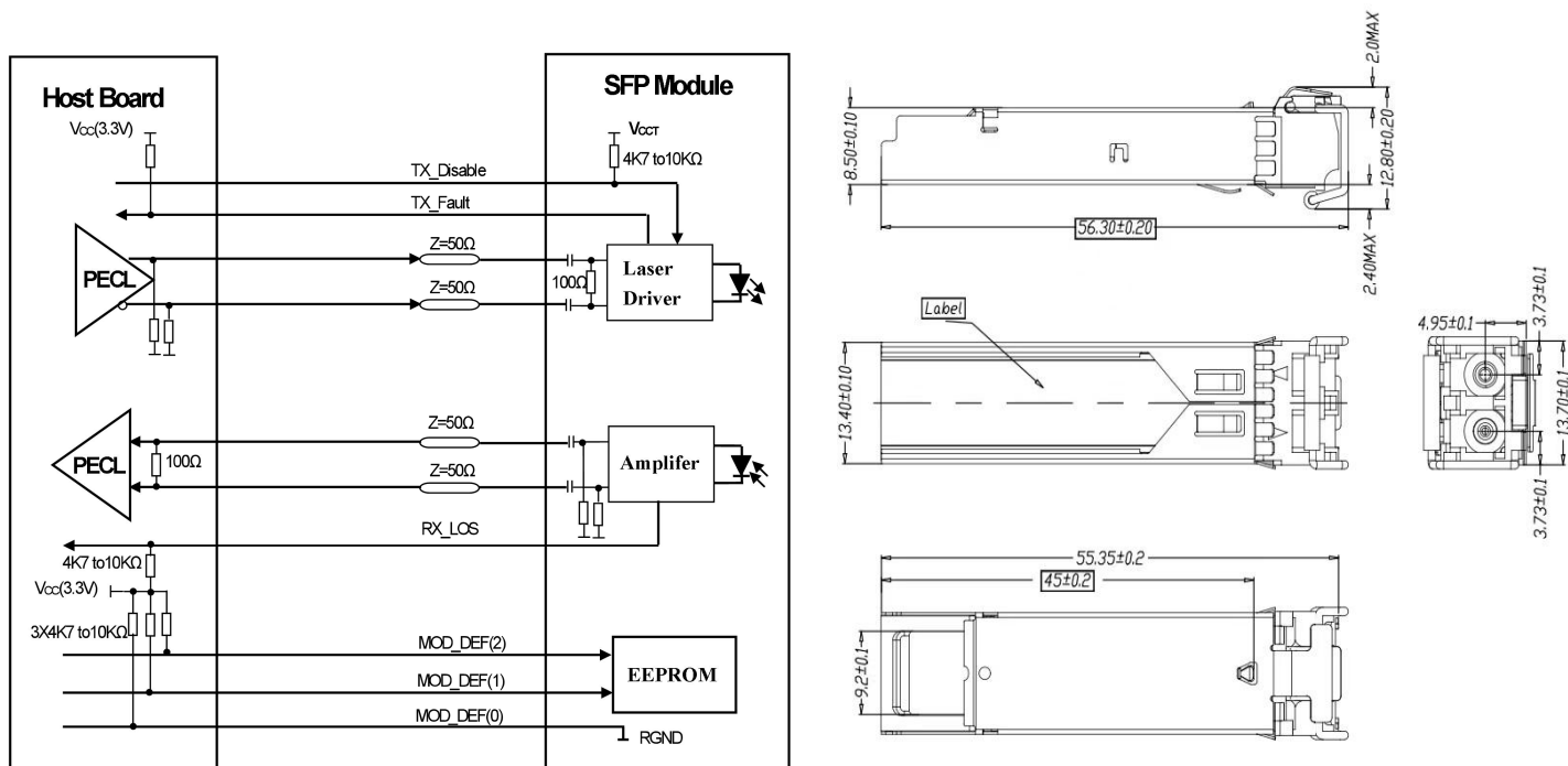
SFP Host Recommended Circuit
