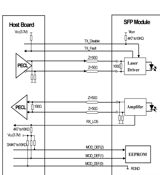
SFP Host Recommended Circuit
