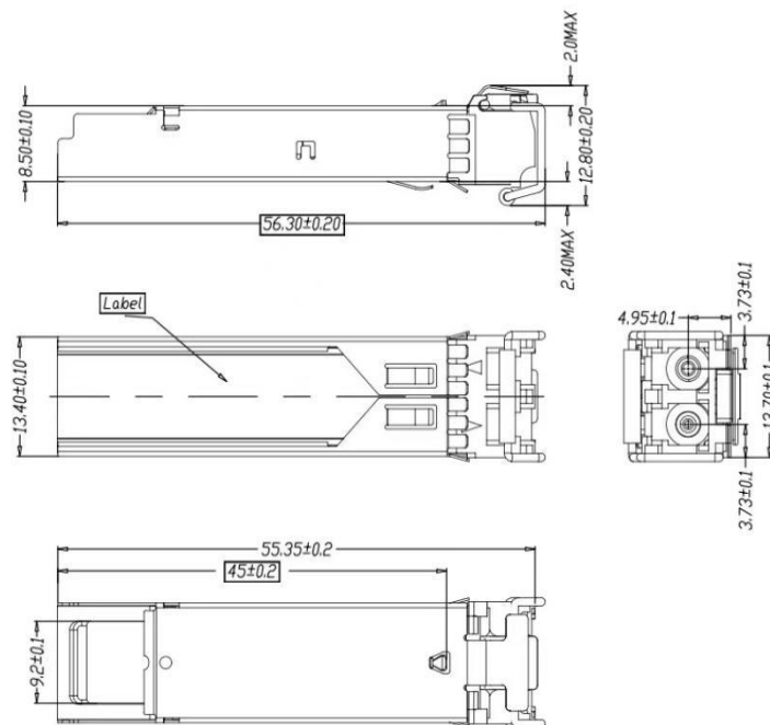
Mechanical Drawing
