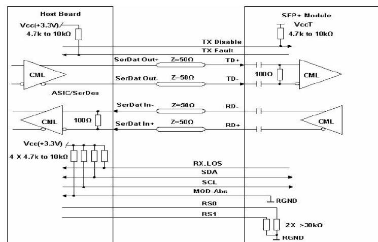
Recommended High-speed Interface Circuit
