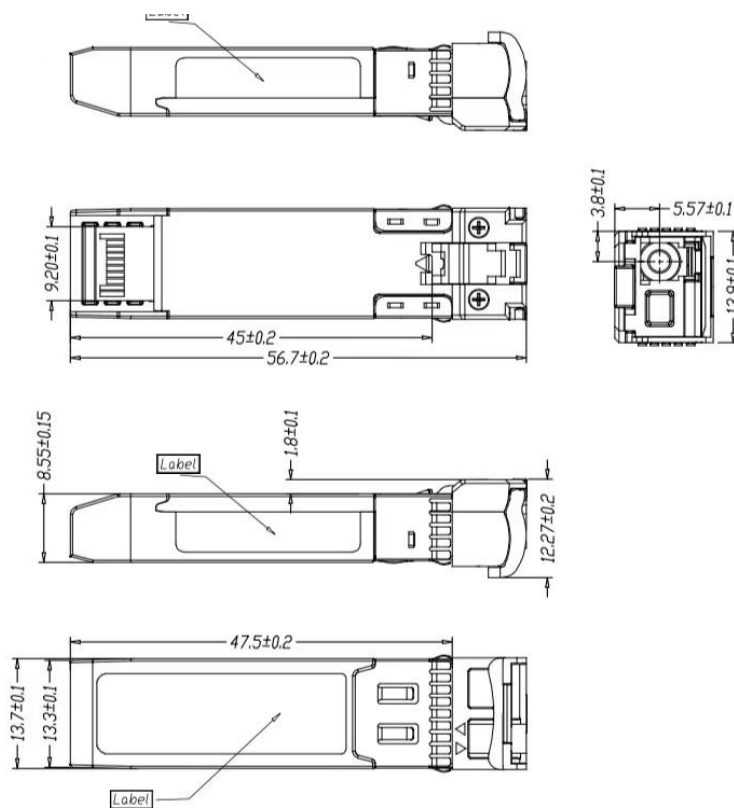
Mechanical Drawing
