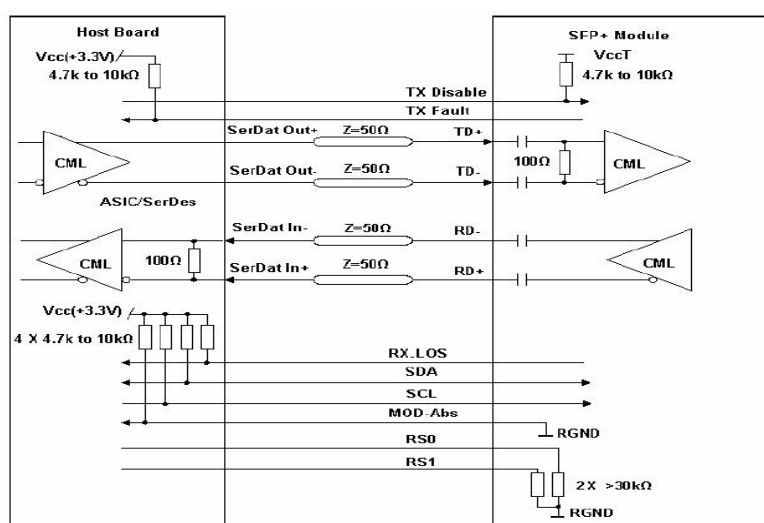
Recommended High-speed Interface Circuit
