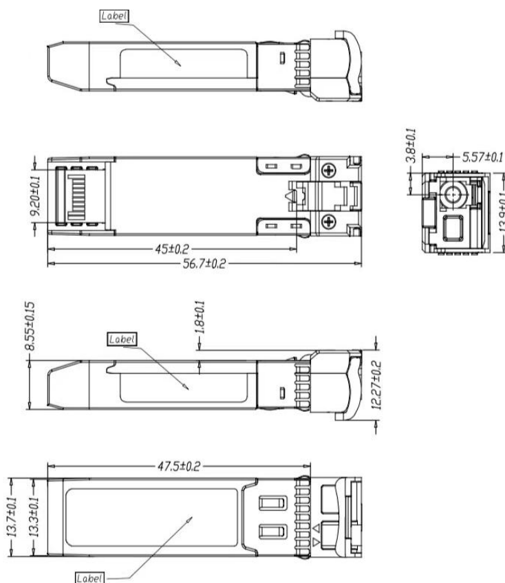
Mechanical Drawing
