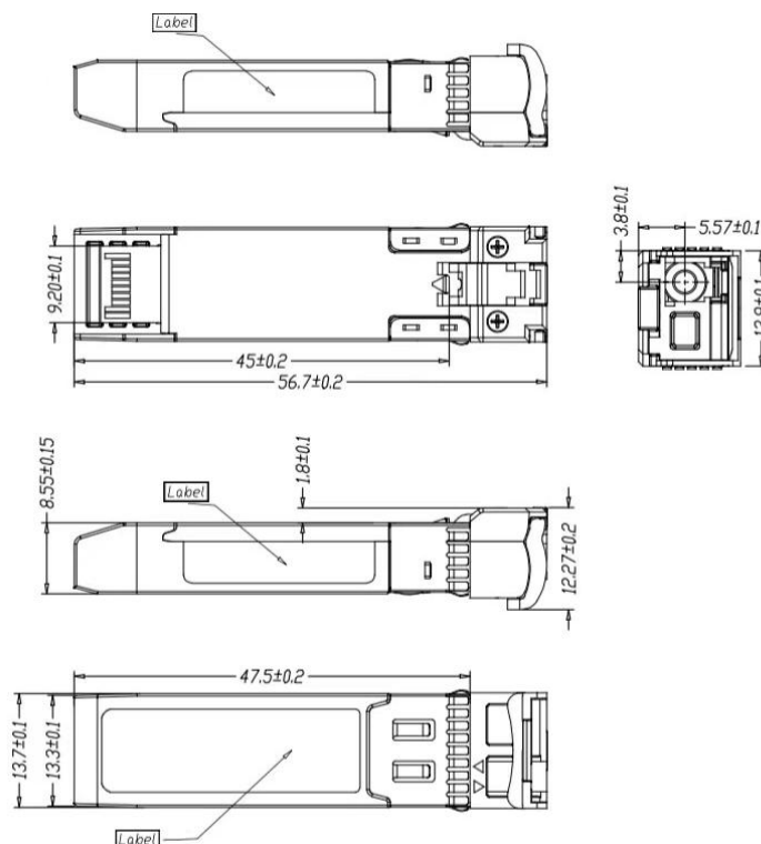
Mechanical Drawing
