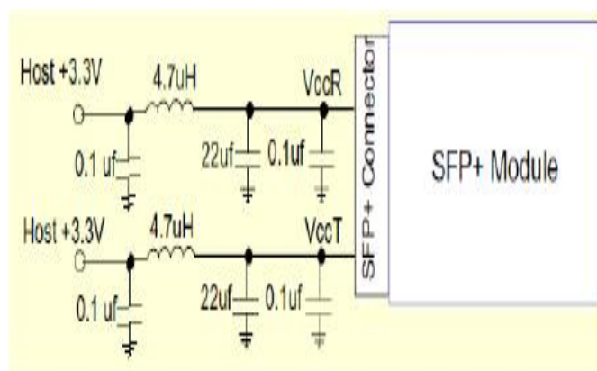
Recommended Host Board Power Supply Circuit
