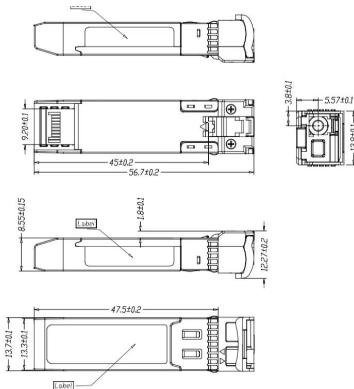
Mechanical Drawin
