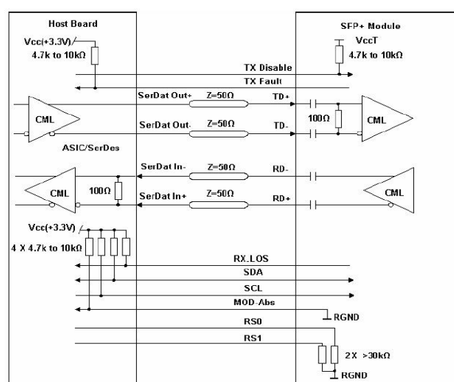
Recommended High-speed Interface Circuit
