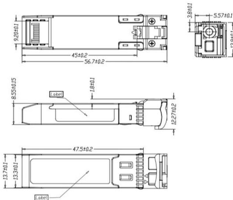
Mechanical Drawing
