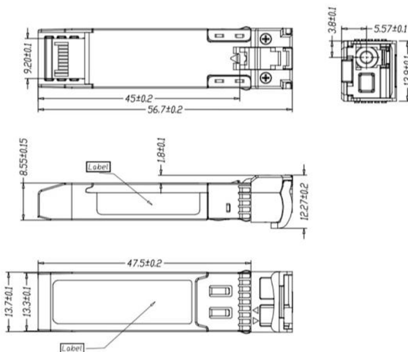
Mechanical Drawing
