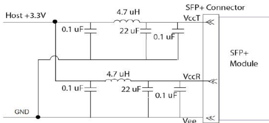
Recommended Host Board Power Supply Circuit
