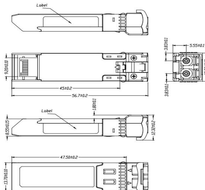
Mechanical Drawing
