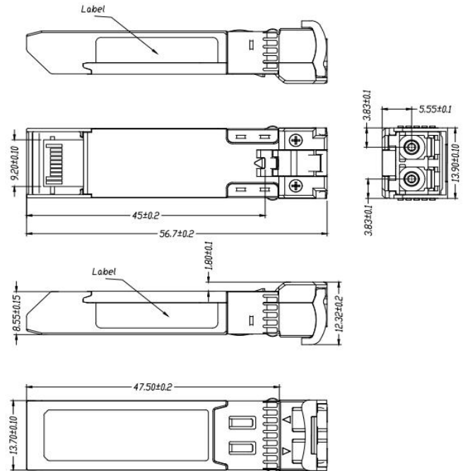
Mechanical Drawing
