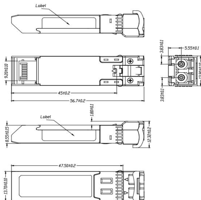
Mechanical Drawing
