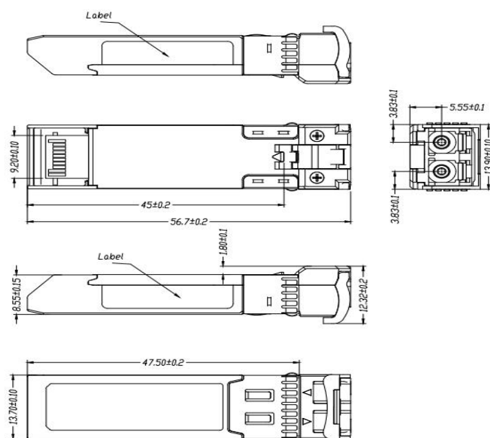
Mechanical Drawing
