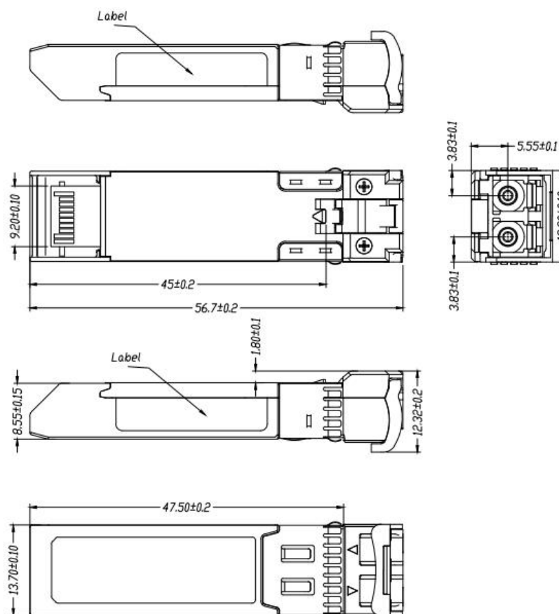
Mechanical Drawing
