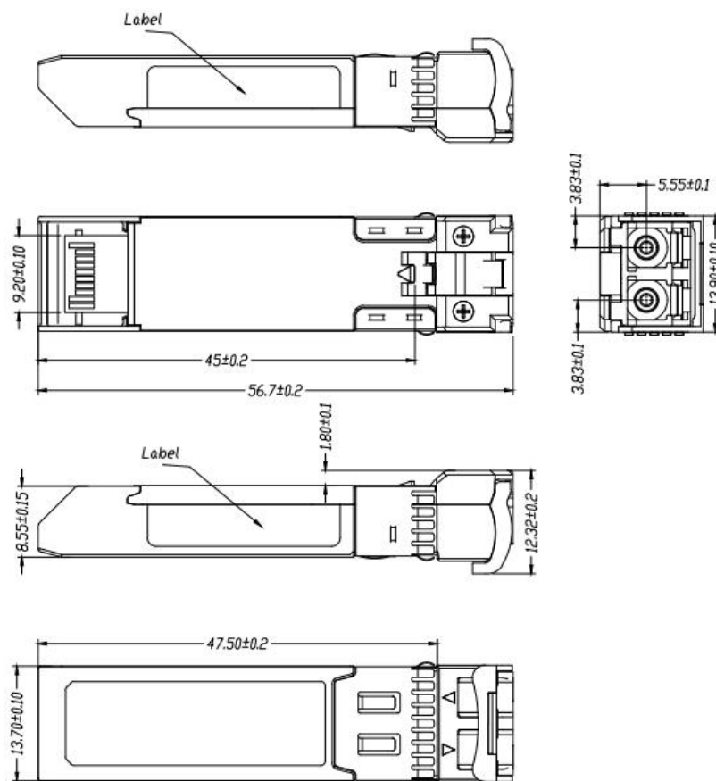
Mechanical Drawing
