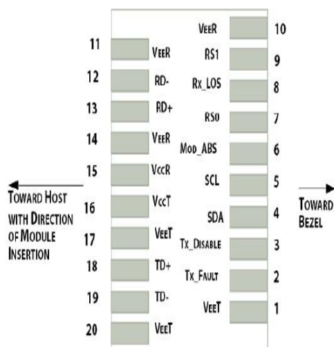
Figure2:Diagram of Host Board Connector Block Pin Numbers and Names
