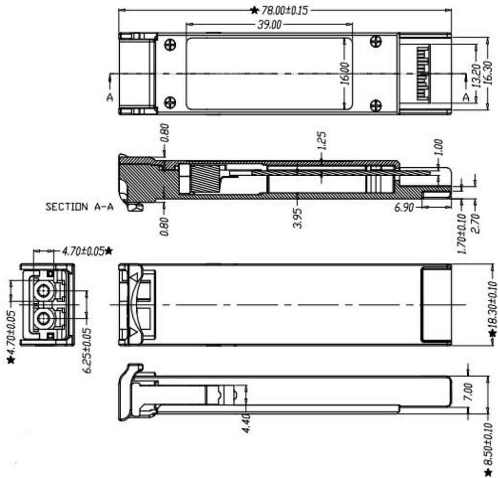
Mechanical Drawing
