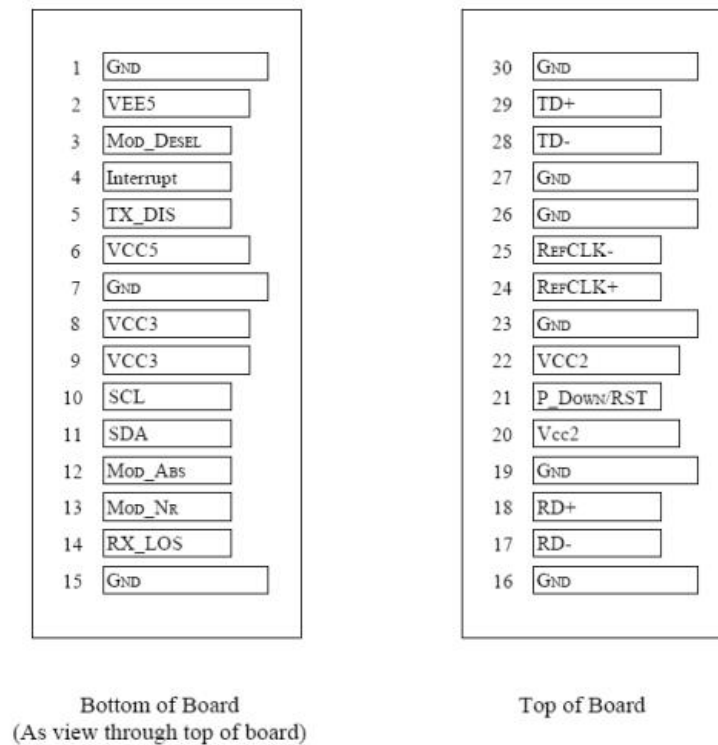
Diagram of Host Board Connector Block Pin Numbers and Names
