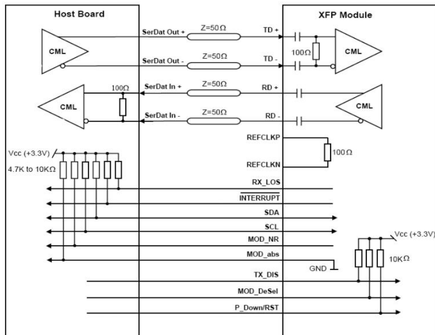
SFP Host Recommended Circuit
